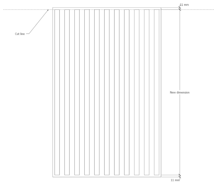
Figure 5. Positioning the new support blade on an HARMONY tile.
