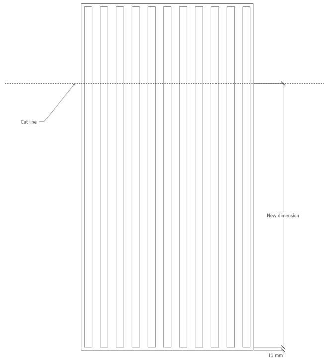
Figure 4. Cut perpendicular to the main blades on an HARMONY tile.
