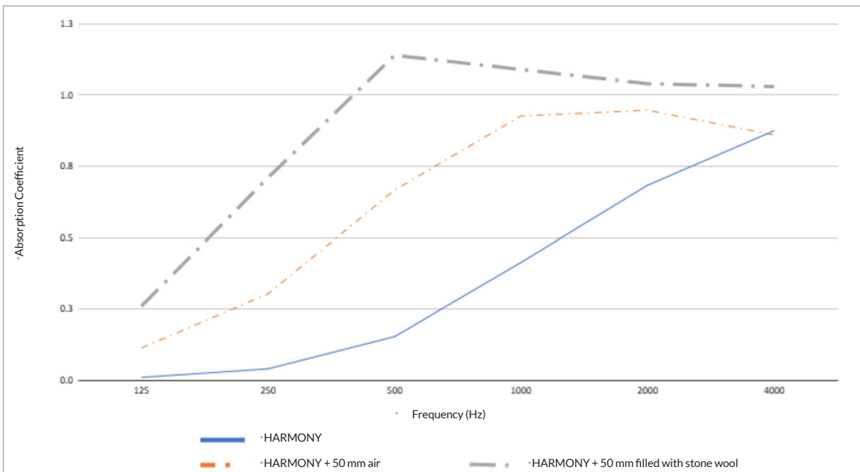
Figure 1. Acoustic performance for HARMONY panel 2713.
