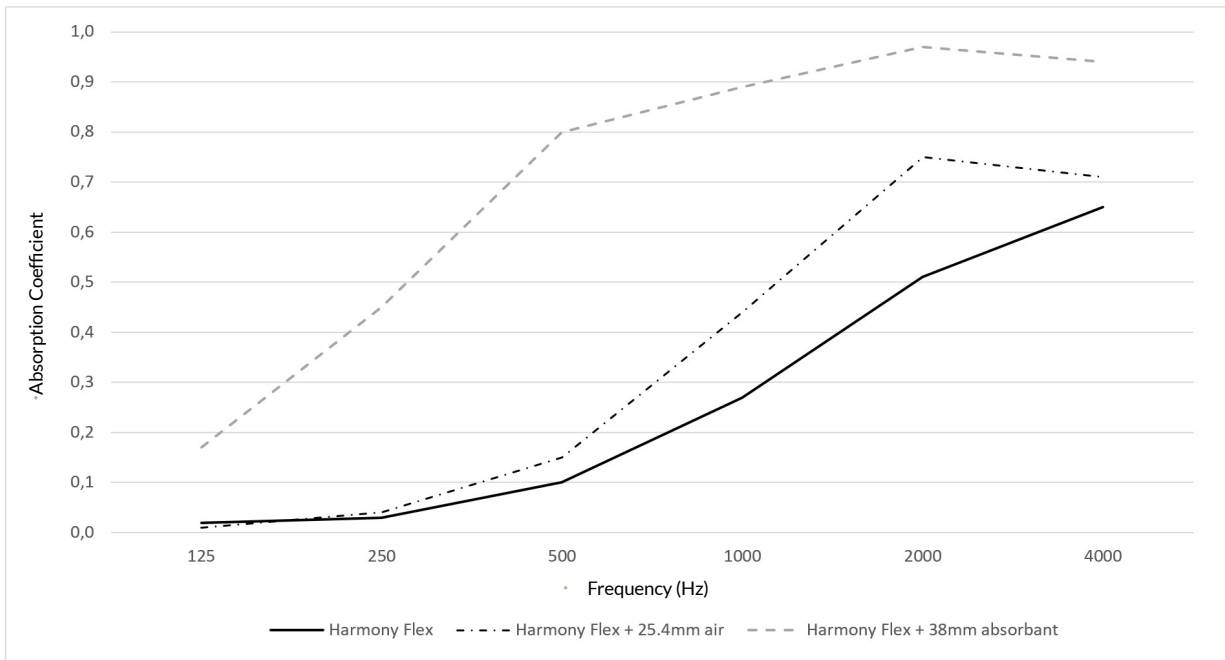
Figure 1. Acoustic performance for HARMONY FLEX panel 2713.
