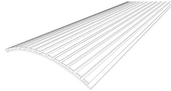
Figure 2. Isometric section view of the HARMONY FLEX acoustical panel 2713.
