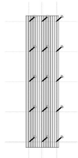
Side-by-side installation
